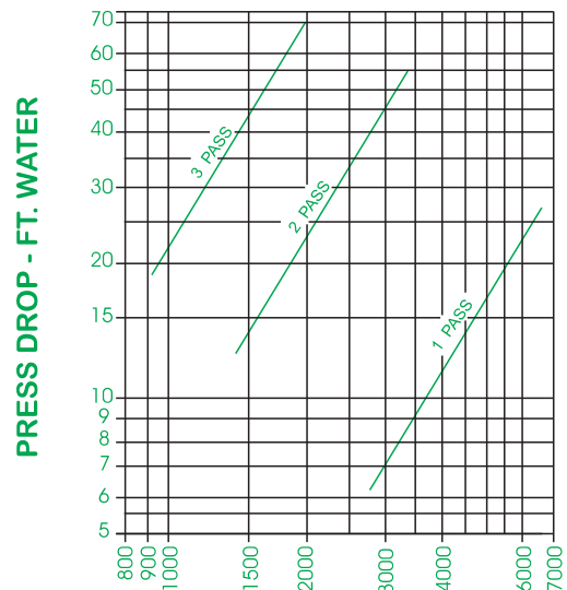
CHILLED WATER
