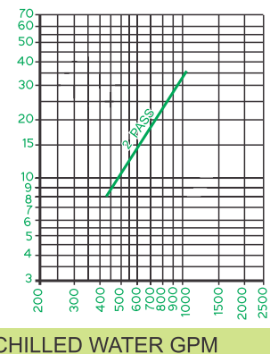
PRESS DROP - FT. WATER
