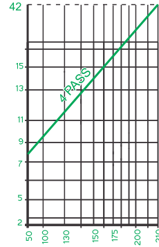
PRESS DROP - FT. WATER
